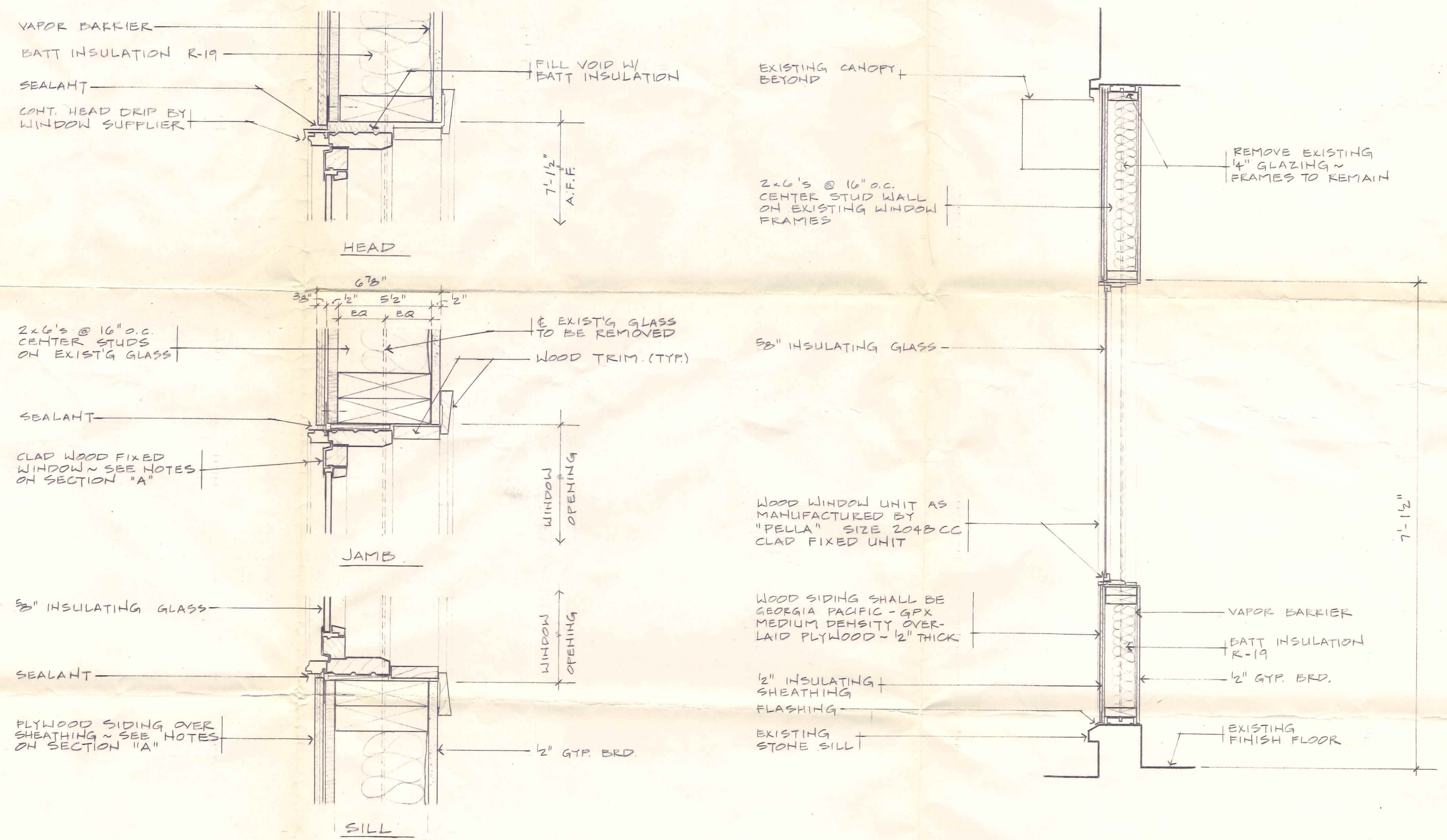
WINDOW DETAILS 3" = 1'-0"
